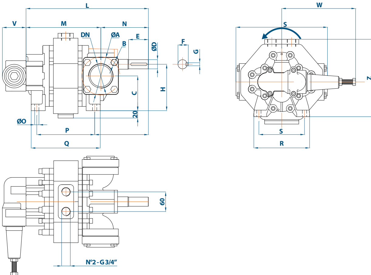
Fig. 515 - BC200 to BC400 dimensional drawing
